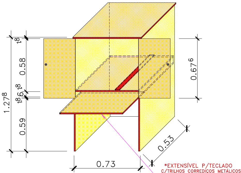
Vista Frontal
